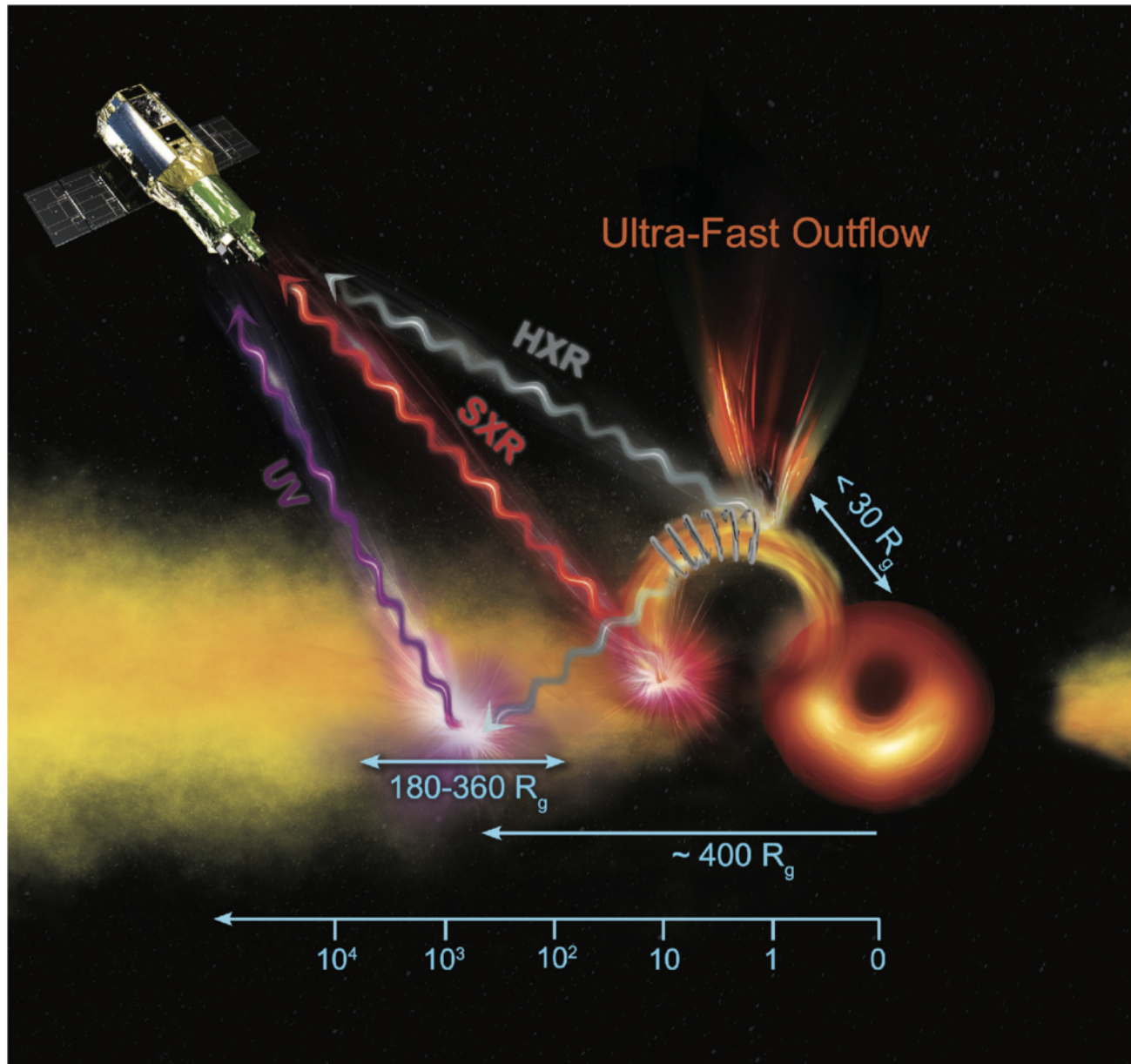
Figure 9. from Gal Vardi et al 2026 Astrophys. J. Lett. 1007 doi:10.3847/2041-8213/ae8f44 https://dx.doi.org/10.3847/2041-8213/ae8f44 © 2026. The Author(s). Published by the American Astronomical Society.
