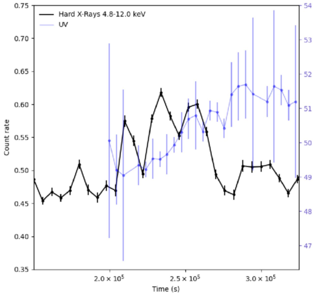
Figure 8. from Gal Vardi et al 2026 Astrophys. J. Lett. 1007 doi:10.3847/2041-8213/ae8f44 https://dx.doi.org/10.3847/2041-8213/ae8f44 © 2026. The Author(s). Published by the American Astronomical Society.
