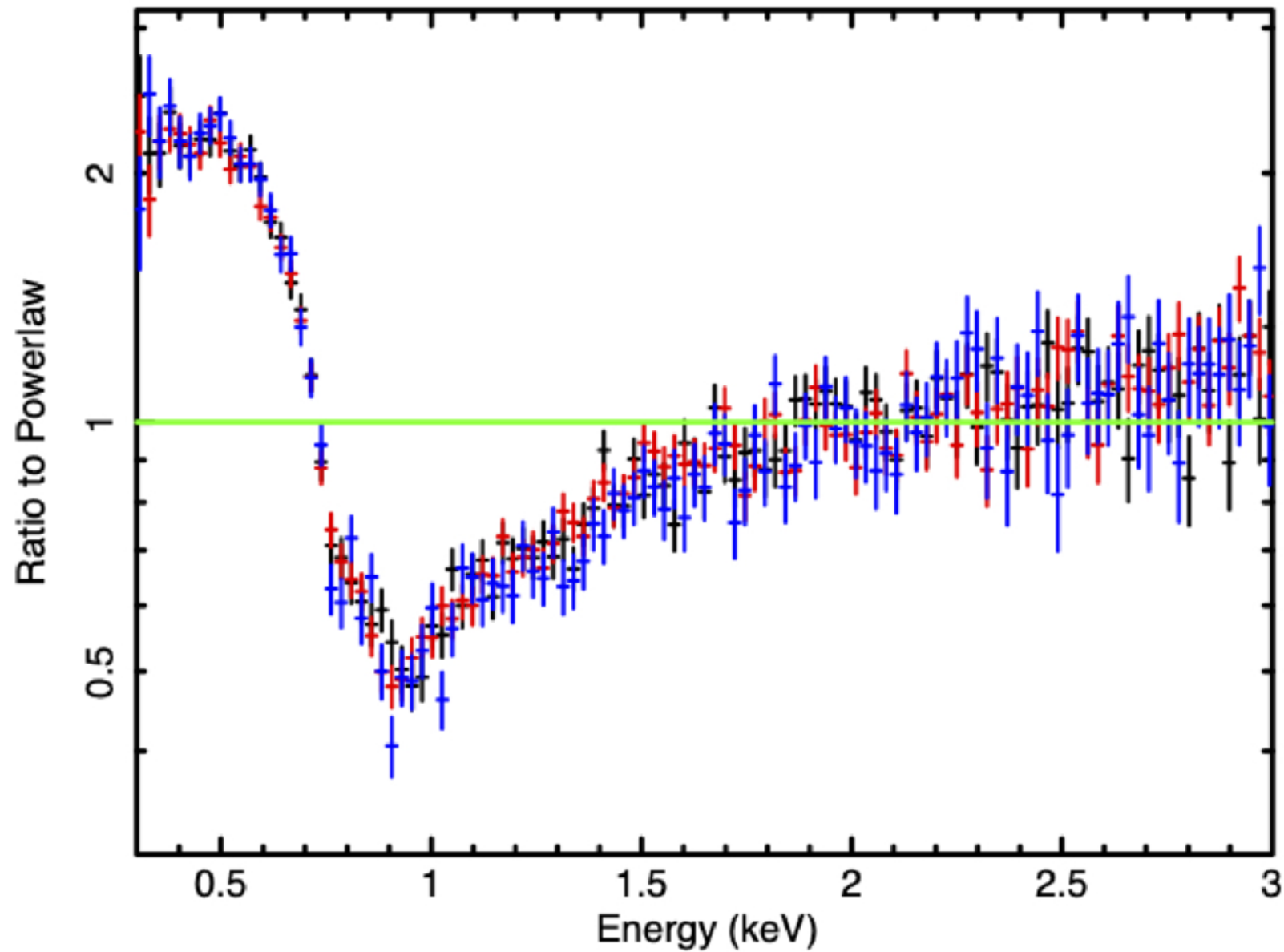
Figure 4. from Gal Vardi et al 2026 Astrophys. J. Lett. 1007 doi:10.3847/2041-8213/ae8f44 https://dx.doi.org/10.3847/2041-8213/ae8f44 © 2026. The Author(s). Published by the American Astronomical Society.
