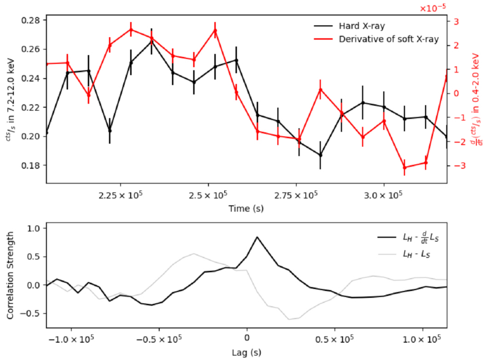
Figure 3. from Gal Vardi et al 2026 Astrophys. J. Lett. 1007 doi:10.3847/2041-8213/ae8f44 https://dx.doi.org/10.3847/2041-8213/ae8f44 © 2026. The Author(s). Published by the American Astronomical Society.
