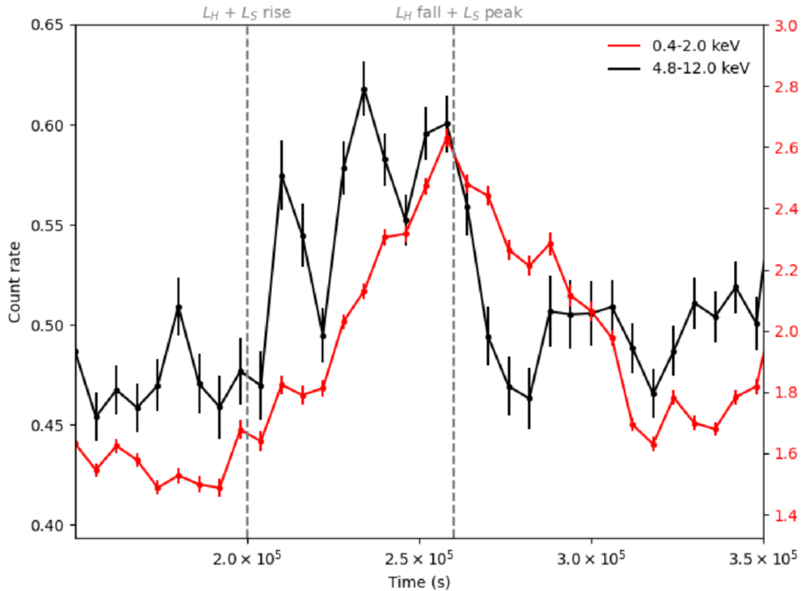
Figure 2. from Gal Vardi et al 2026 Astrophys. J. Lett. 1007 doi:10.3847/2041-8213/ae8f44 https://dx.doi.org/10.3847/2041-8213/ae8f44 © 2026. The Author(s). Published by the American Astronomical Society.
