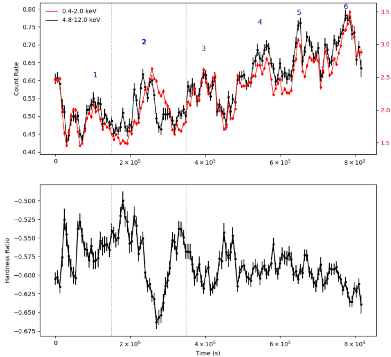
Figure 1. from Gal Vardi et al 2026 Astrophys. J. Lett. 1007 doi:10.3847/2041-8213/ae8f44 https://dx.doi.org/10.3847/2041-8213/ae8f44 © 2026. The Author(s). Published by the American Astronomical Society.
