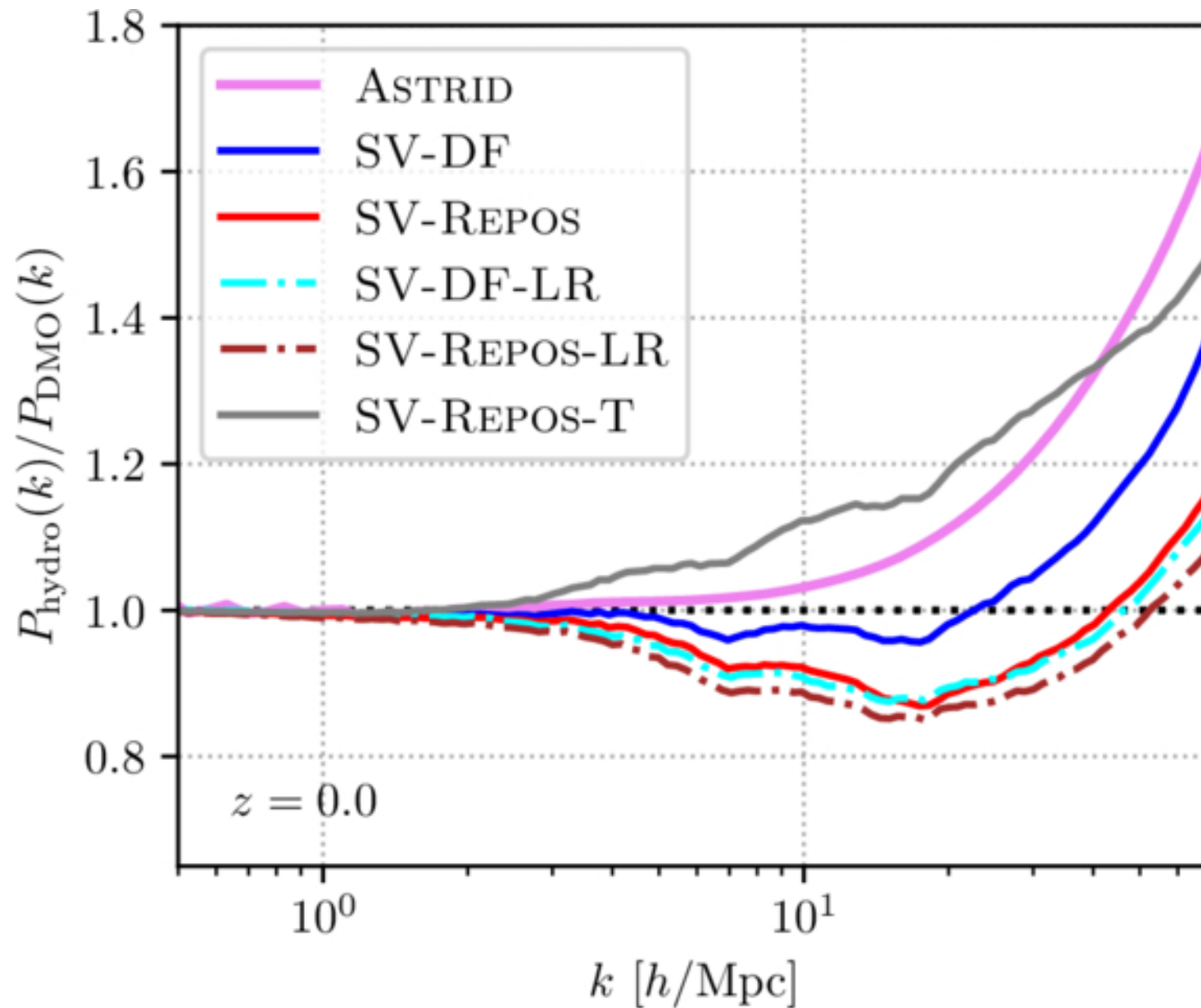
Figure B1. from Yanhui Yang et al 2026 Astrophys. J. Lett. 1007 doi:10.3847/2041-8213/ae8dc6 https://dx.doi.org/10.3847/2041-8213/ae8dc6 © 2026. The Author(s). Published by the American Astronomical Society.
