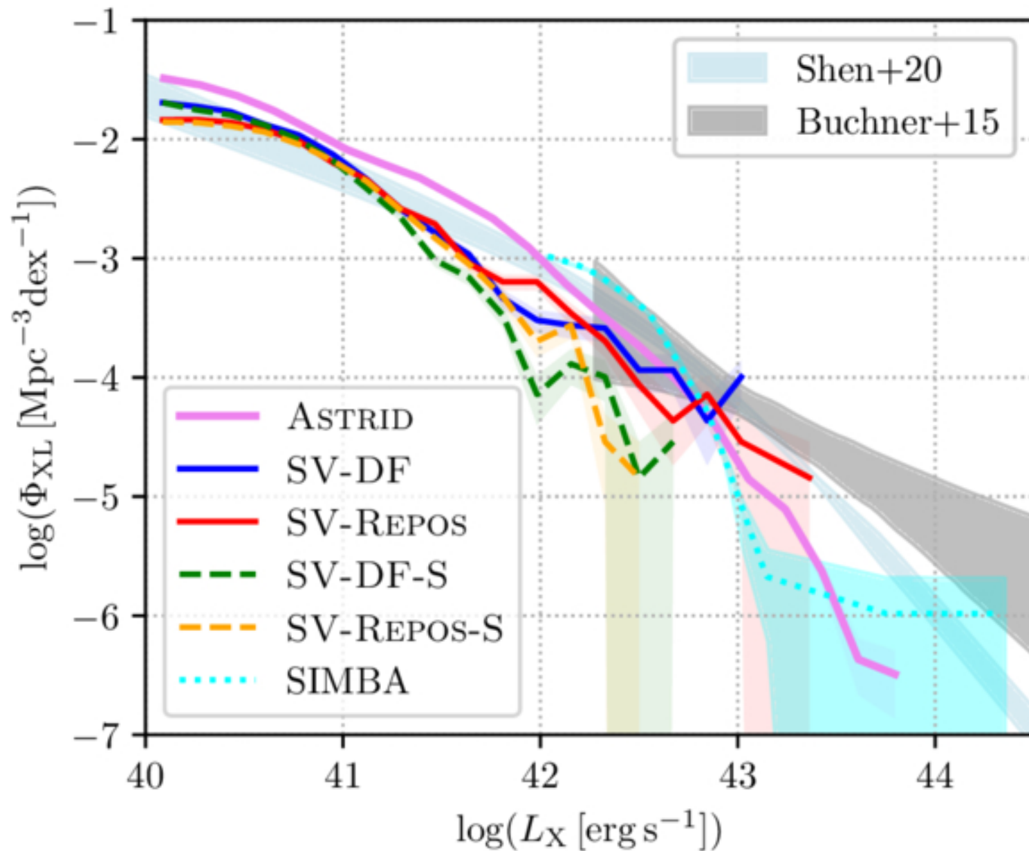
Figure 4. from Yanhui Yang et al 2026 Astrophys. J. Lett. 1007 doi:10.3847/2041-8213/ae8dc6 https://dx.doi.org/10.3847/2041-8213/ae8dc6 © 2026. The Author(s). Published by the American Astronomical Society.
