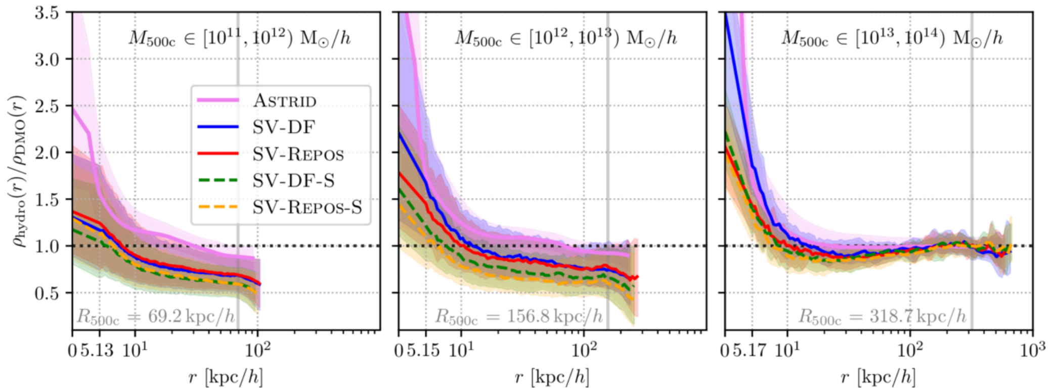
Figure 2. from Yanhui Yang et al 2026 Astrophys. J. Lett. 1007 doi:10.3847/2041-8213/ae8dc6 https://dx.doi.org/10.3847/2041-8213/ae8dc6 © 2026. The Author(s). Published by the American Astronomical Society.
