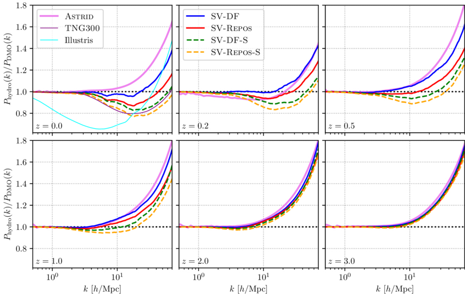
Figure 1. from Yanhui Yang et al 2026 Astrophys. J. Lett. 1007 doi:10.3847/2041-8213/ae8dc6 https://dx.doi.org/10.3847/2041-8213/ae8dc6 © 2026. The Author(s). Published by the American Astronomical Society.
