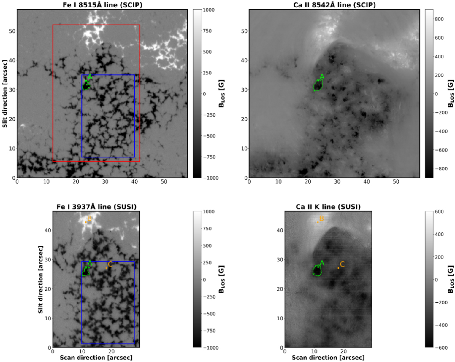
Figure 2. from Iñigo Juanikorena Berasategi et al 2026 Astrophys. J. Lett. 1007 doi:10.3847/2041-8213/ae8dc4 https://dx.doi.org/10.3847/2041-8213/ae8dc4 © 2026. The Author(s). Published by the American Astronomical Society.
