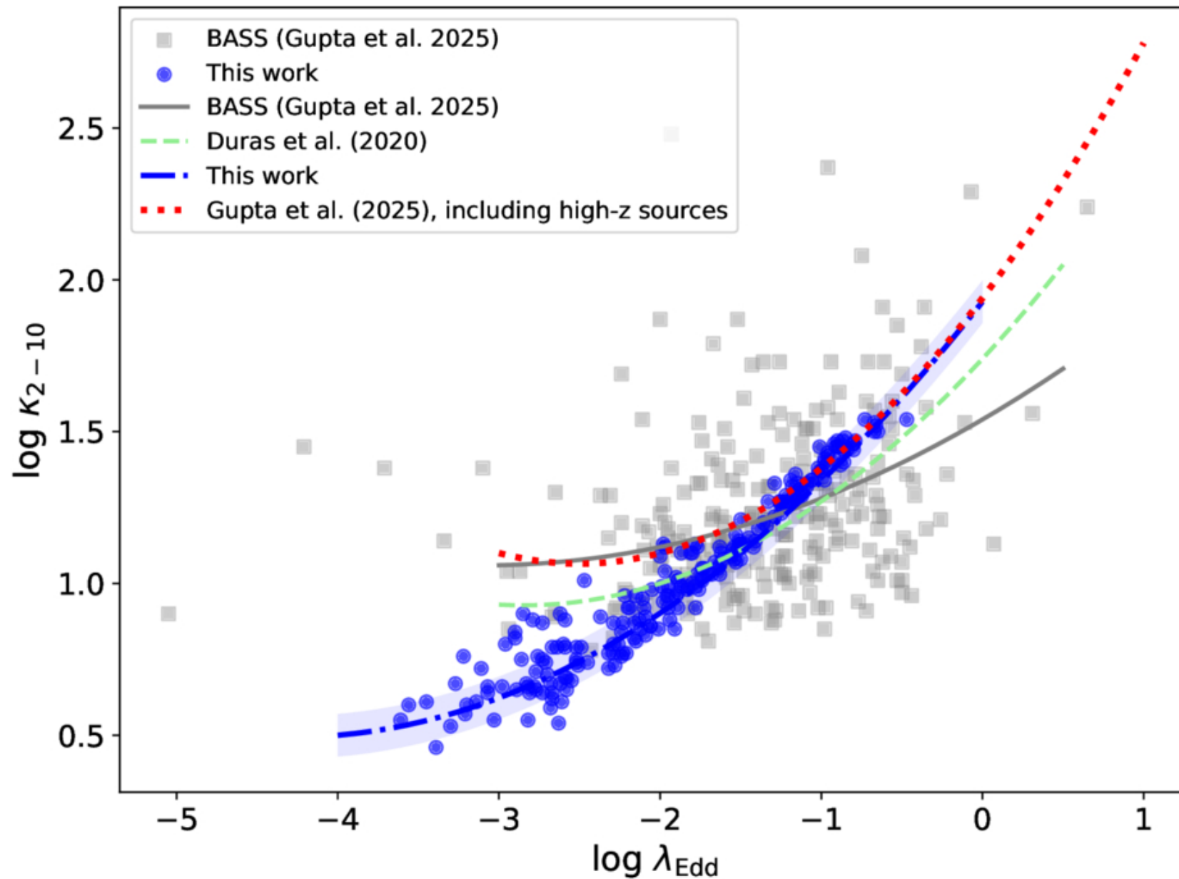
Figure 4. from Arghajit Jana et al 2026 Astrophys. J. Lett. 1007 doi:10.3847/2041-8213/ae8dc1 https://dx.doi.org/10.3847/2041-8213/ae8dc1 © 2026. The Author(s). Published by the American Astronomical Society.
