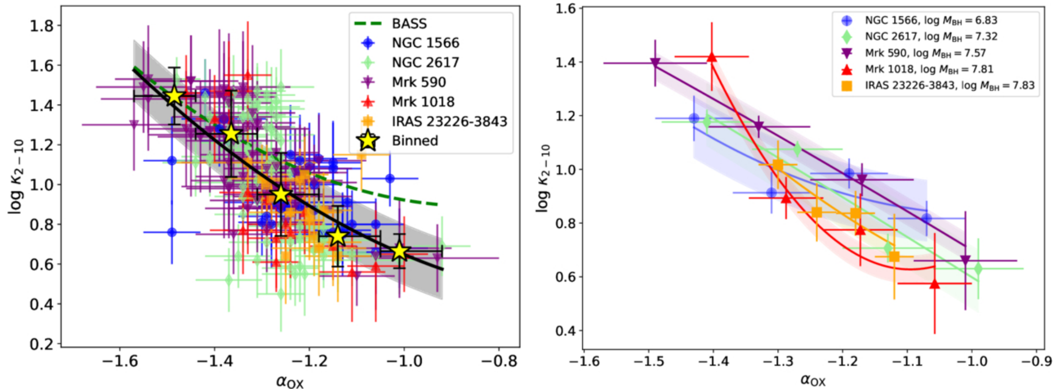
Figure 3. from Arghajit Jana et al 2026 Astrophys. J. Lett. 1007 doi:10.3847/2041-8213/ae8dc1 https://dx.doi.org/10.3847/2041-8213/ae8dc1 © 2026. The Author(s). Published by the American Astronomical Society.
