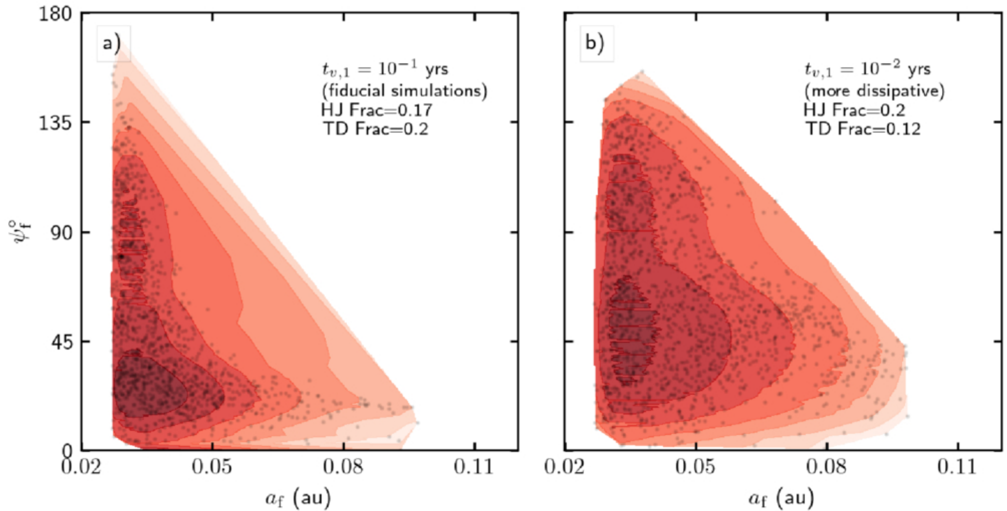
Figure 7. from Hareesh Gautham Bhaskar et al 2026 Astrophys. J. Lett. 1007 doi:10.3847/2041-8213/ae8dbc https://dx.doi.org/10.3847/2041-8213/ae8dbc © 2026. The Author(s). Published by the American Astronomical Society.
