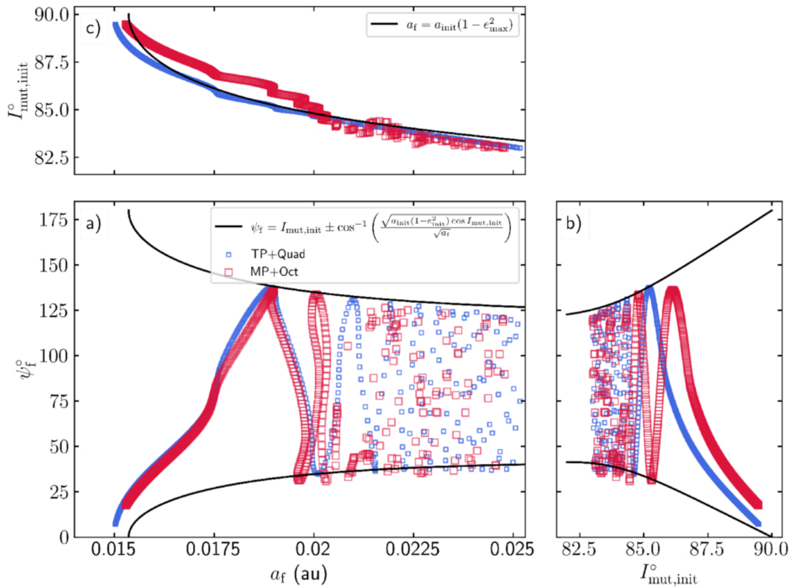
Figure 6. from Hareesh Gautham Bhaskar et al 2026 Astrophys. J. Lett. 1007 doi:10.3847/2041-8213/ae8dbc https://dx.doi.org/10.3847/2041-8213/ae8dbc © 2026. The Author(s). Published by the American Astronomical Society.
