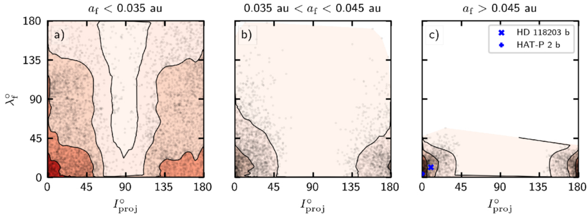
Figure 5. from Hareesh Gautham Bhaskar et al 2026 Astrophys. J. Lett. 1007 doi:10.3847/2041-8213/ae8dbc https://dx.doi.org/10.3847/2041-8213/ae8dbc © 2026. The Author(s). Published by the American Astronomical Society.
