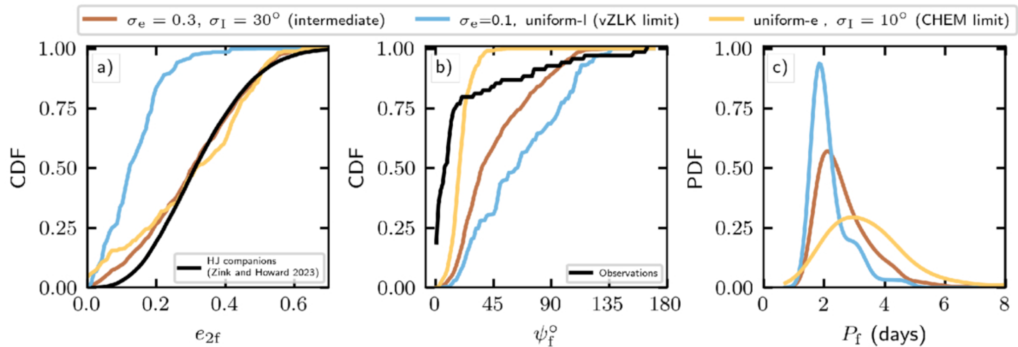
Figure 4. from Hareesh Gautham Bhaskar et al 2026 Astrophys. J. Lett. 1007 doi:10.3847/2041-8213/ae8dbc https://dx.doi.org/10.3847/2041-8213/ae8dbc © 2026. The Author(s). Published by the American Astronomical Society.
