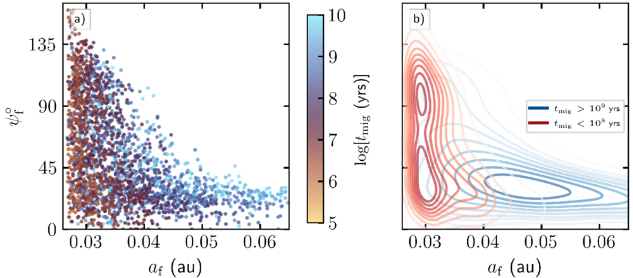
Figure 2. from Hareesh Gautham Bhaskar et al 2026 Astrophys. J. Lett. 1007 doi:10.3847/2041-8213/ae8dbc https://dx.doi.org/10.3847/2041-8213/ae8dbc © 2026. The Author(s). Published by the American Astronomical Society.
