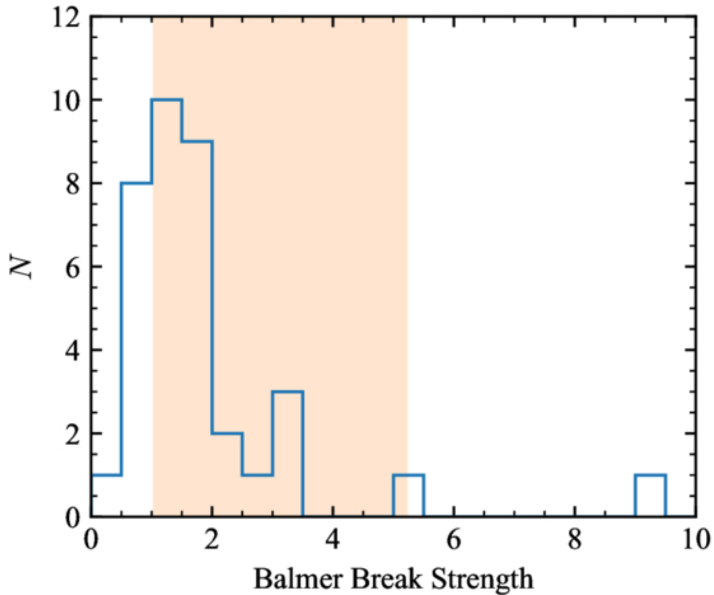
Figure 4. from Jun-Rong Liu et al 2026 Astrophys. J. Lett. 1007 doi:10.3847/2041-8213/ae8dba https://dx.doi.org/10.3847/2041-8213/ae8dba © 2026. The Author(s). Published by the American Astronomical Society.
