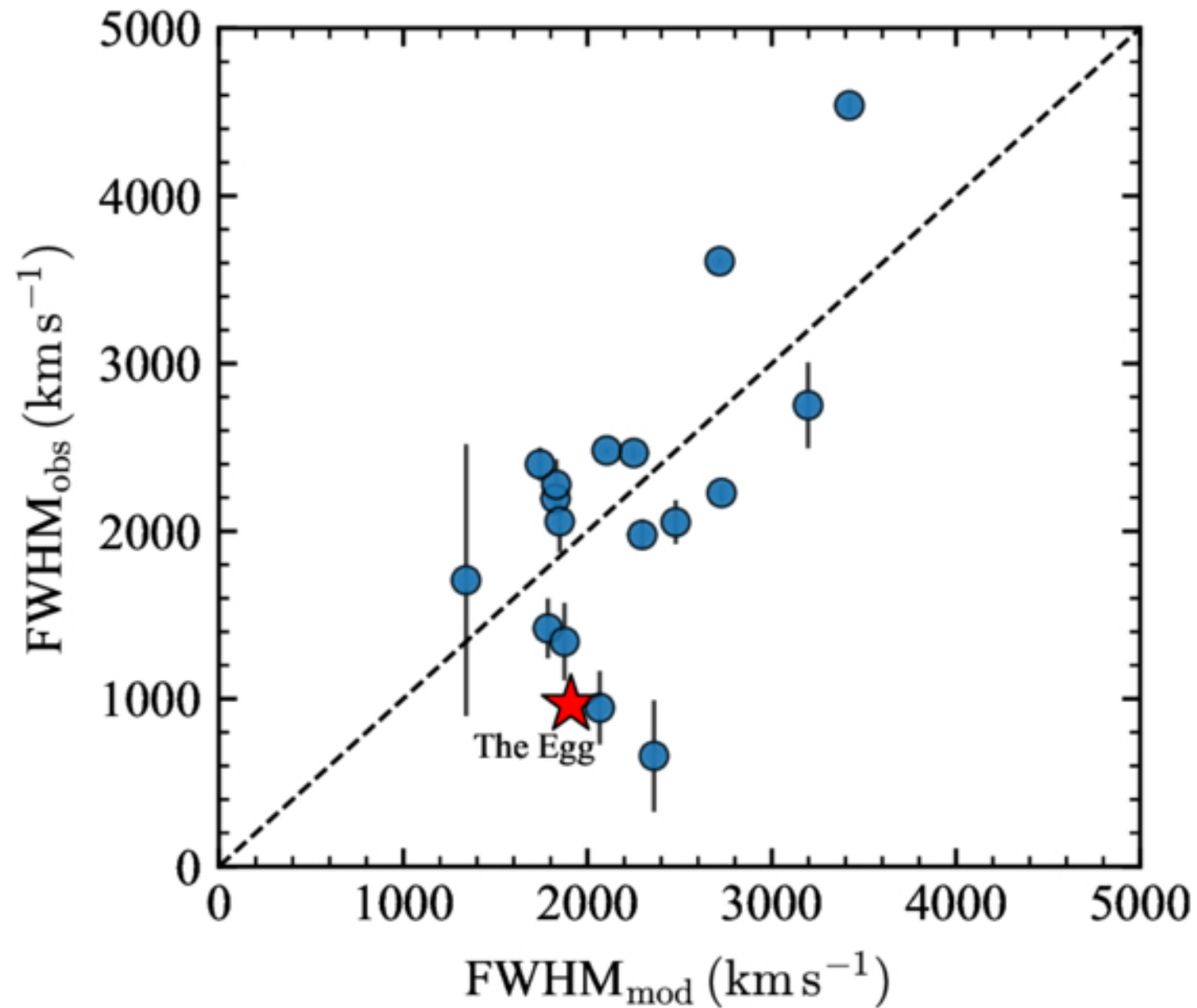
Figure 3. from Jun-Rong Liu et al 2026 Astrophys. J. Lett. 1007 doi:10.3847/2041-8213/ae8dba https://dx.doi.org/10.3847/2041-8213/ae8dba © 2026. The Author(s). Published by the American Astronomical Society.
