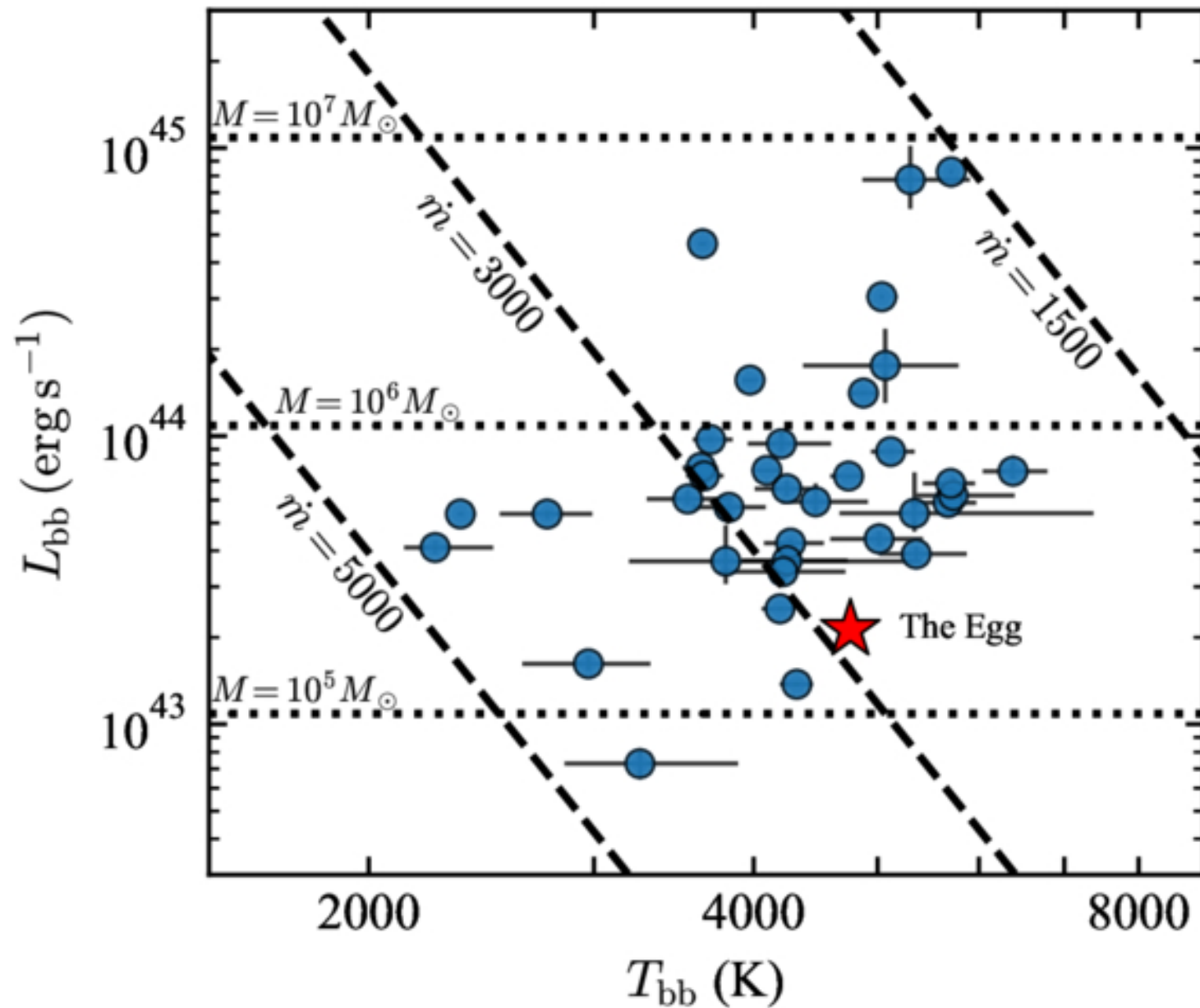
Figure 2. from Jun-Rong Liu et al 2026 Astrophys. J. Lett. 1007 doi:10.3847/2041-8213/ae8dba https://dx.doi.org/10.3847/2041-8213/ae8dba © 2026. The Author(s). Published by the American Astronomical Society.
