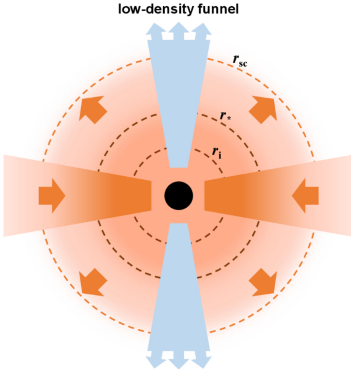
Figure 1. from Jun-Rong Liu et al 2026 Astrophys. J. Lett. 1007 doi:10.3847/2041-8213/ae8dba https://dx.doi.org/10.3847/2041-8213/ae8dba © 2026. The Author(s). Published by the American Astronomical Society.
