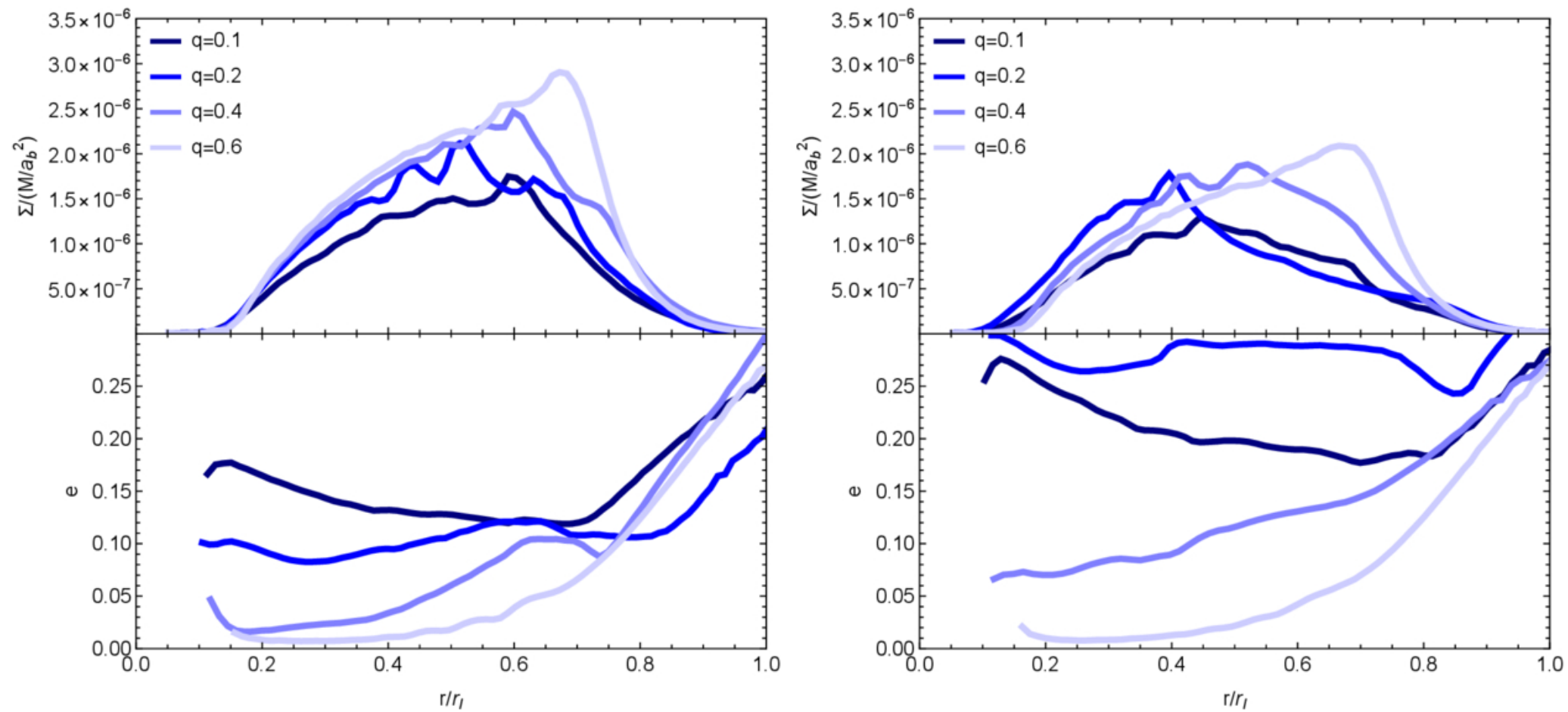
Figure 2. from Rebecca G. Martin et al 2026 Astrophys. J. Lett. 1007 doi:10.3847/2041-8213/ae8da4 https://dx.doi.org/10.3847/2041-8213/ae8da4 © 2026. The Author(s). Published by the American Astronomical Society.
