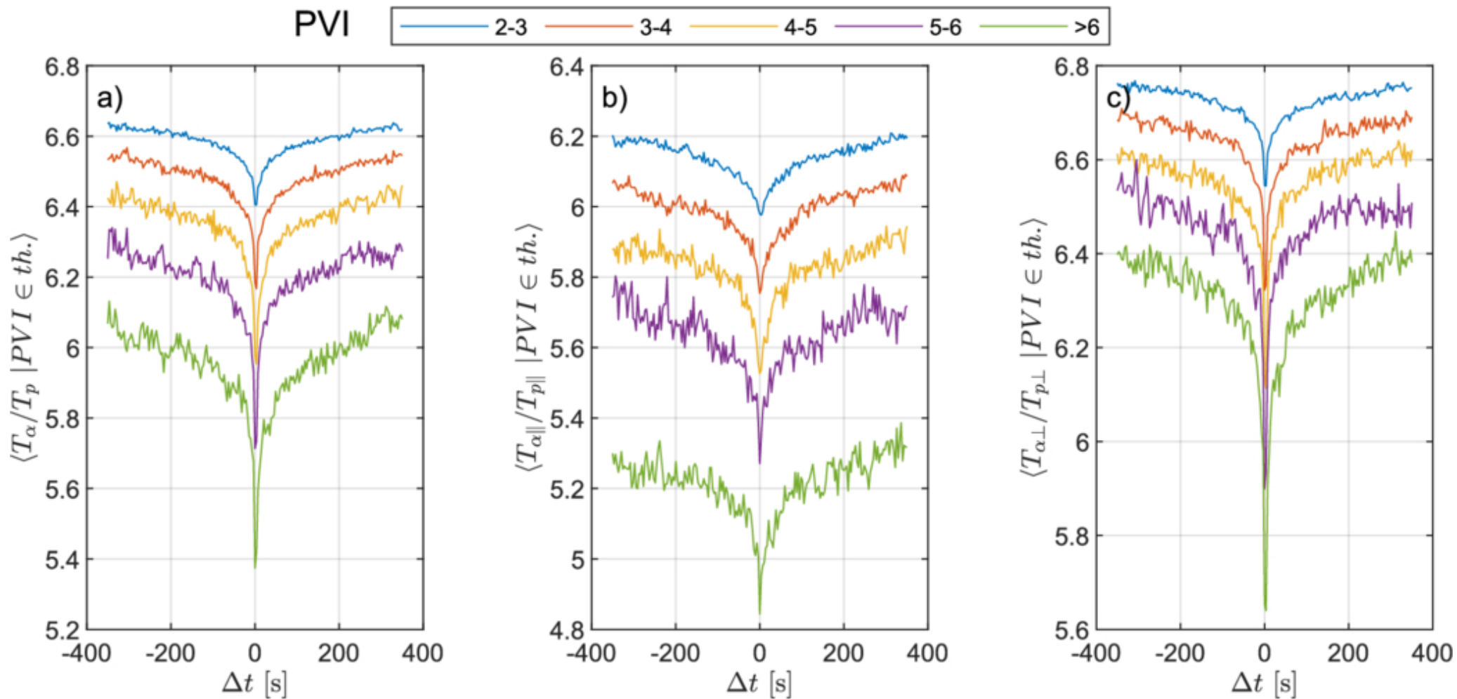
Figure 3. from Jiayang Xi et al 2026 Astrophys. J. Lett. 1007 doi:10.3847/2041-8213/ae8d1c https://dx.doi.org/10.3847/2041-8213/ae8d1c © 2026. The Author(s). Published by the American Astronomical Society.
