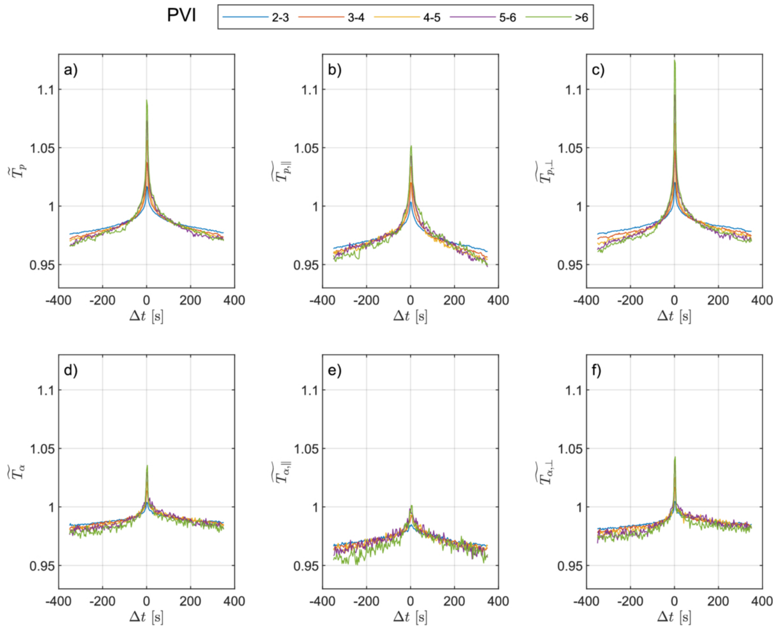
Figure 2. from Jiayang Xi et al 2026 Astrophys. J. Lett. 1007 doi:10.3847/2041-8213/ae8d1c https://dx.doi.org/10.3847/2041-8213/ae8d1c © 2026. The Author(s). Published by the American Astronomical Society.
