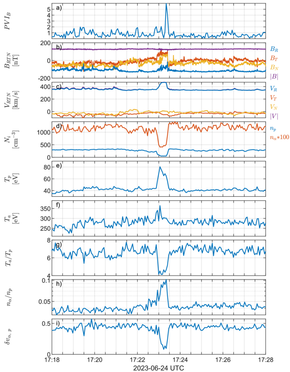
Figure 1. from Jiayang Xi et al 2026 Astrophys. J. Lett. 1007 doi:10.3847/2041-8213/ae8d1c https://dx.doi.org/10.3847/2041-8213/ae8d1c © 2026. The Author(s). Published by the American Astronomical Society.
