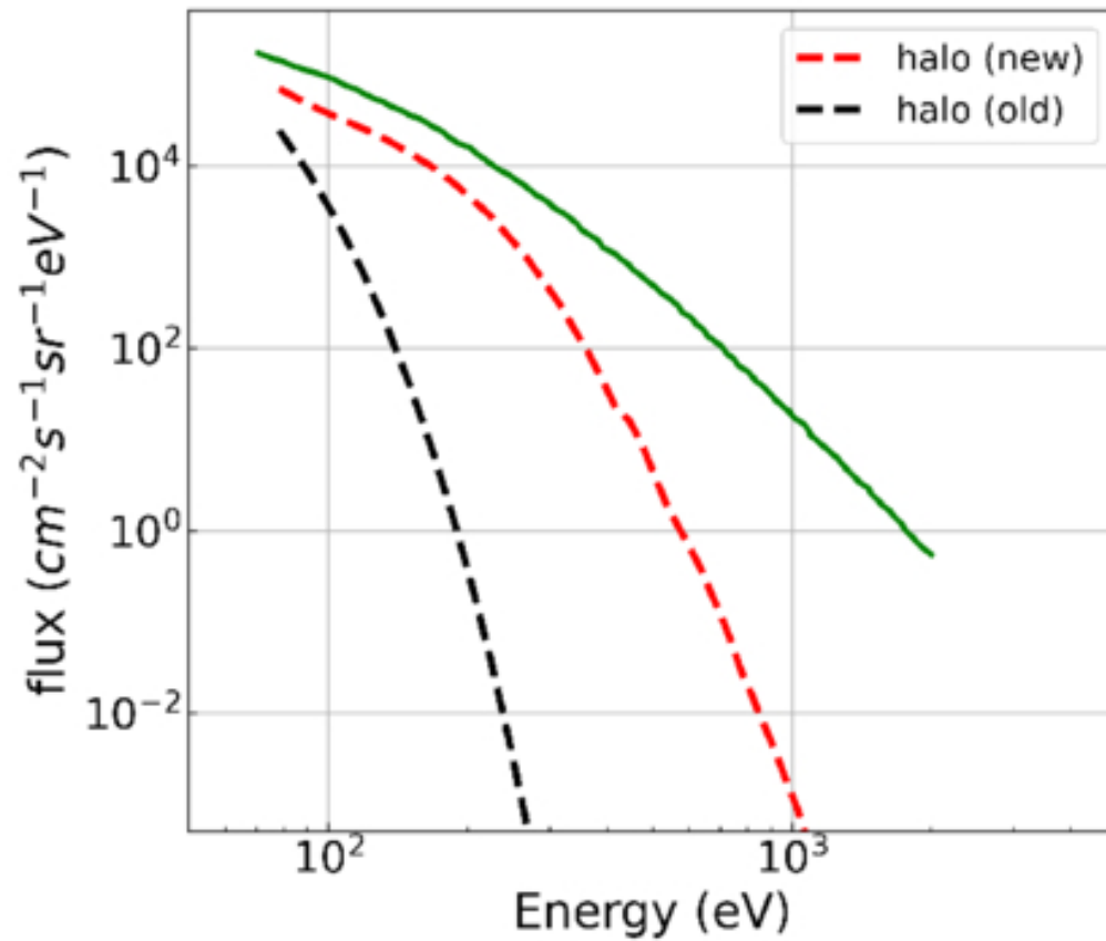
Figure 4. from Bofeng Tang et al 2026 Astrophys. J. Lett. 1006 doi:10.3847/2041-8213/ae8d17 https://dx.doi.org/10.3847/2041-8213/ae8d17 © 2026. The Author(s). Published by the American Astronomical Society.
