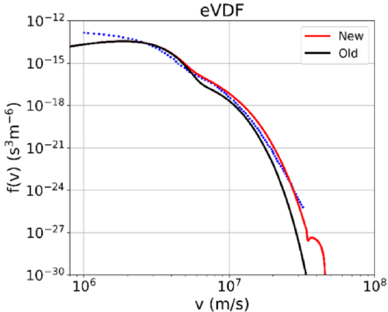
Figure 3. from Bofeng Tang et al 2026 Astrophys. J. Lett. 1006 doi:10.3847/2041-8213/ae8d17 https://dx.doi.org/10.3847/2041-8213/ae8d17 © 2026. The Author(s). Published by the American Astronomical Society.
