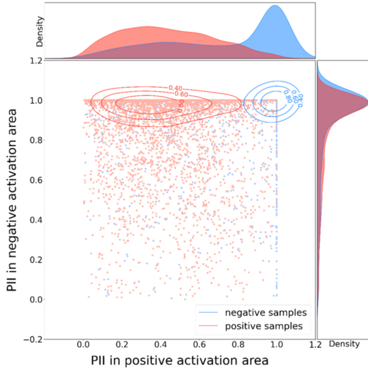
Figure 6. from Z. Zheng et al 2026 Astrophys. J. Lett. 1008 doi:10.3847/2041-8213/ae8d12 https://dx.doi.org/10.3847/2041-8213/ae8d12 © 2026. The Author(s). Published by the American Astronomical Society.
