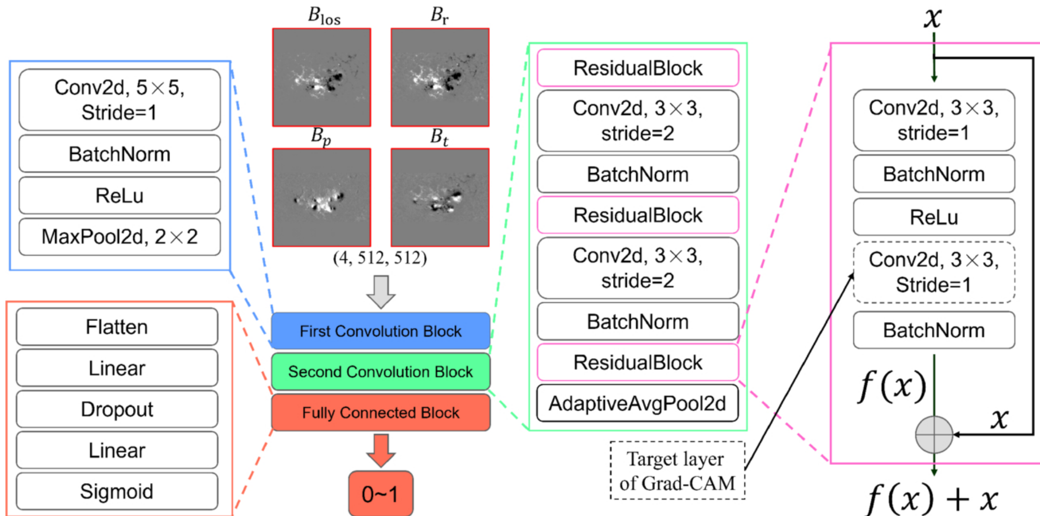
Figure 4. from Z. Zheng et al 2026 Astrophys. J. Lett. 1008 doi:10.3847/2041-8213/ae8d12 https://dx.doi.org/10.3847/2041-8213/ae8d12 © 2026. The Author(s). Published by the American Astronomical Society.
