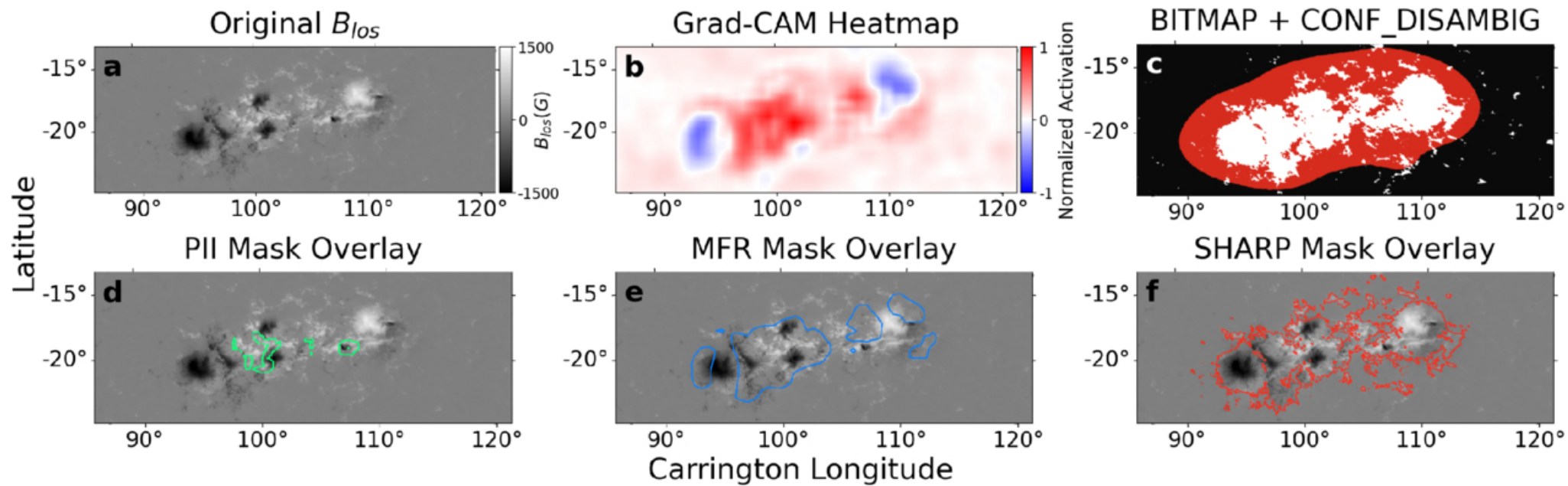
Figure 3. from Z. Zheng et al 2026 Astrophys. J. Lett. 1008 doi:10.3847/2041-8213/ae8d12 https://dx.doi.org/10.3847/2041-8213/ae8d12 © 2026. The Author(s). Published by the American Astronomical Society.
