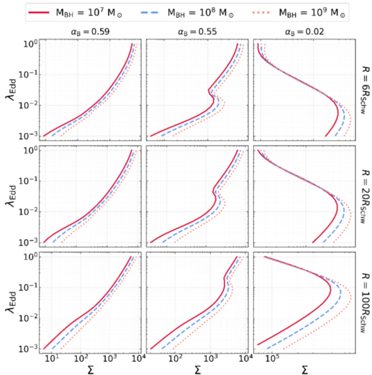
Figure 2. from Marios Kouzlis et al 2026 Astrophys. J. Lett. 1007 doi:10.3847/2041-8213/ae8d11 https://dx.doi.org/10.3847/2041-8213/ae8d11 © 2026. The Author(s). Published by the American Astronomical Society.
