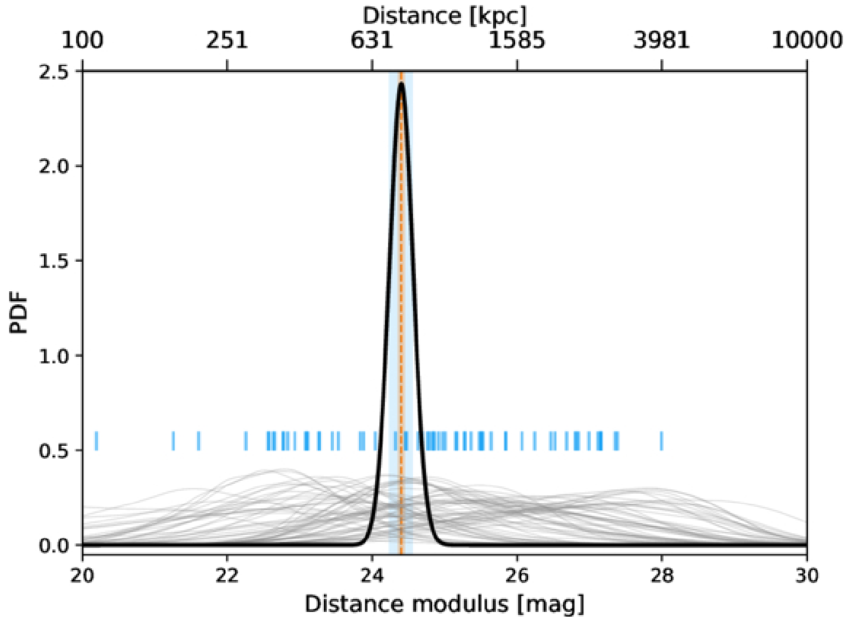
Figure 4. from Ignacio Martín-Navarro et al 2026 Astrophys. J. Lett. 1006 doi:10.3847/2041-8213/ae8d10 https://dx.doi.org/10.3847/2041-8213/ae8d10 © 2026. The Author(s). Published by the American Astronomical Society.
