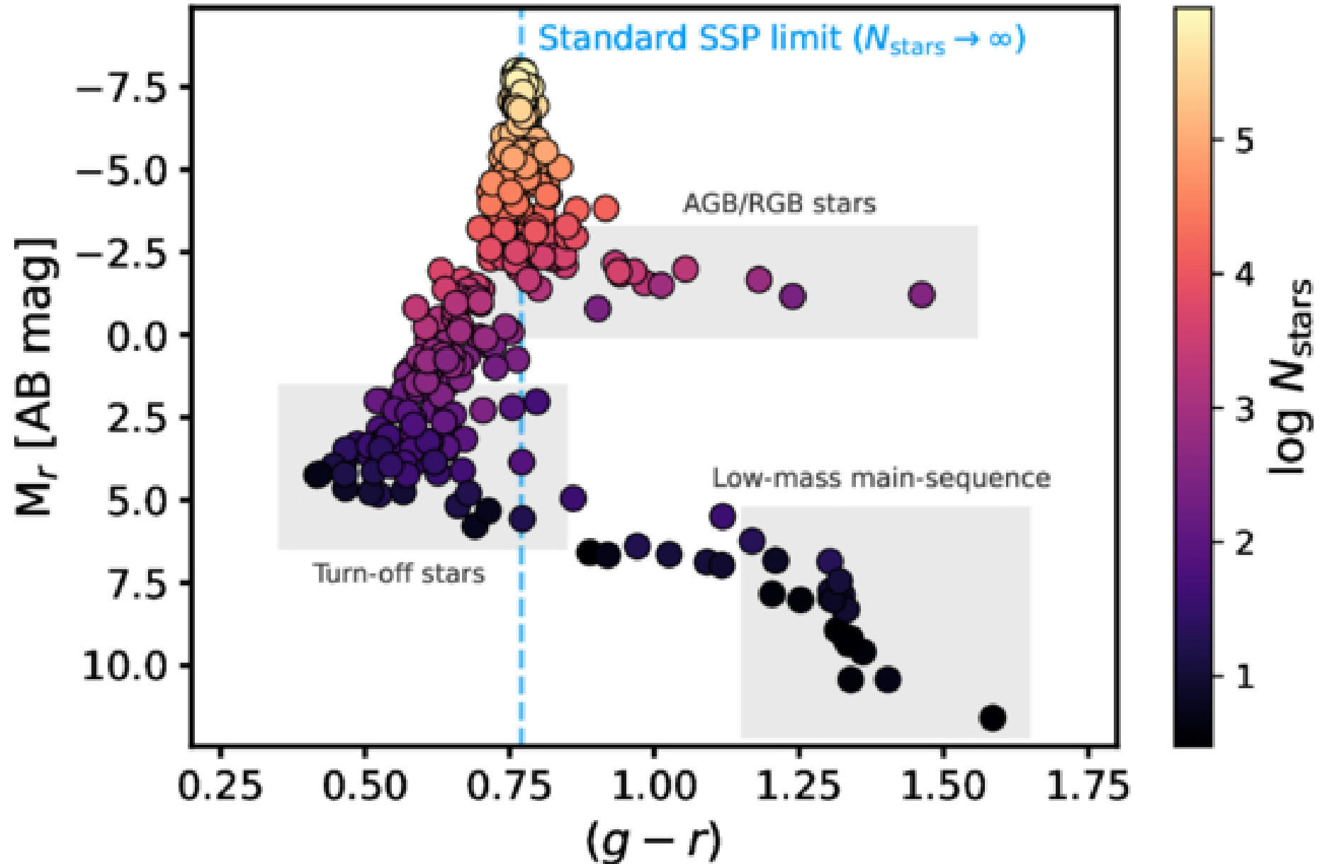
Figure 1. from Ignacio Martín-Navarro et al 2026 Astrophys. J. Lett. 1006 doi:10.3847/2041-8213/ae8d10 https://dx.doi.org/10.3847/2041-8213/ae8d10 © 2026. The Author(s). Published by the American Astronomical Society.
