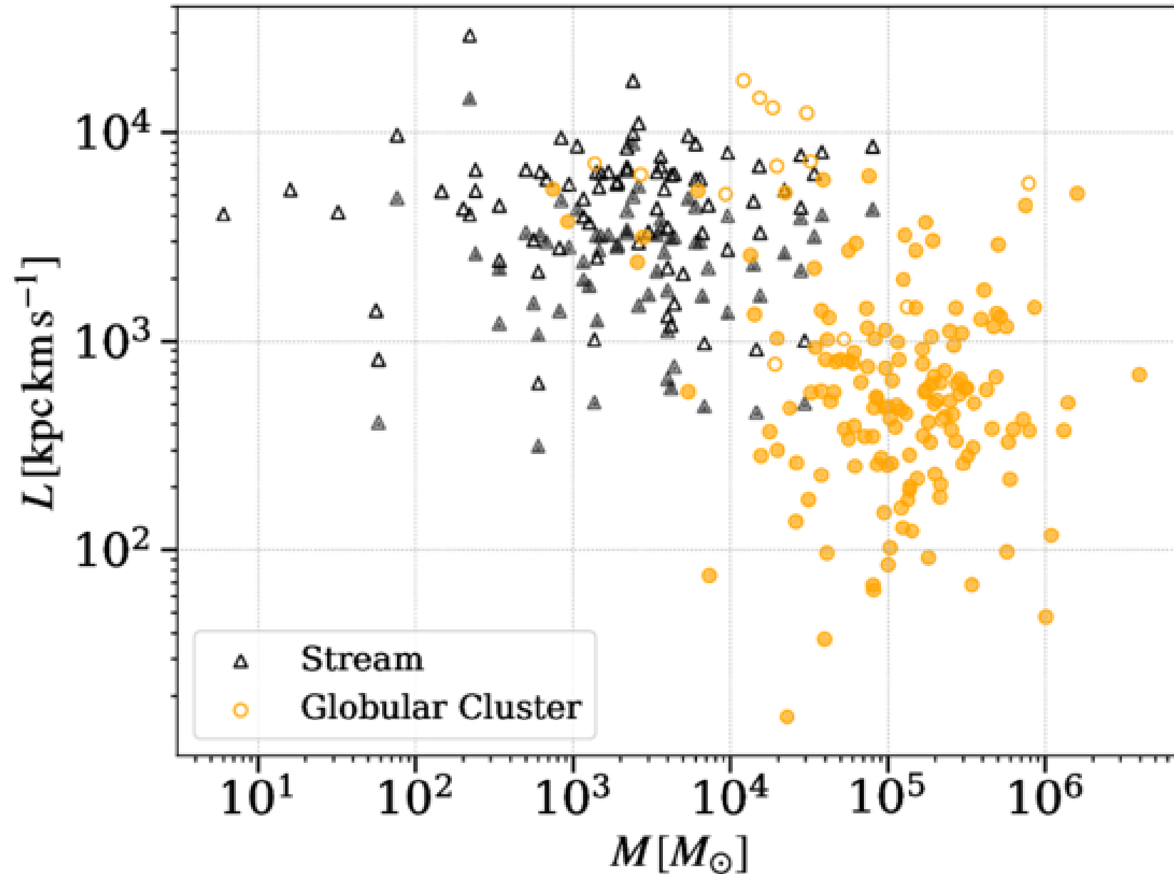
Figure 9. from Claire S. Ye and Raymond G. Carlberg 2026 Astrophys. J. Lett. 1007 doi:10.3847/2041-8213/ae8d0f https://dx.doi.org/10.3847/2041-8213/ae8d0f © 2026. The Author(s). Published by the American Astronomical Society.
