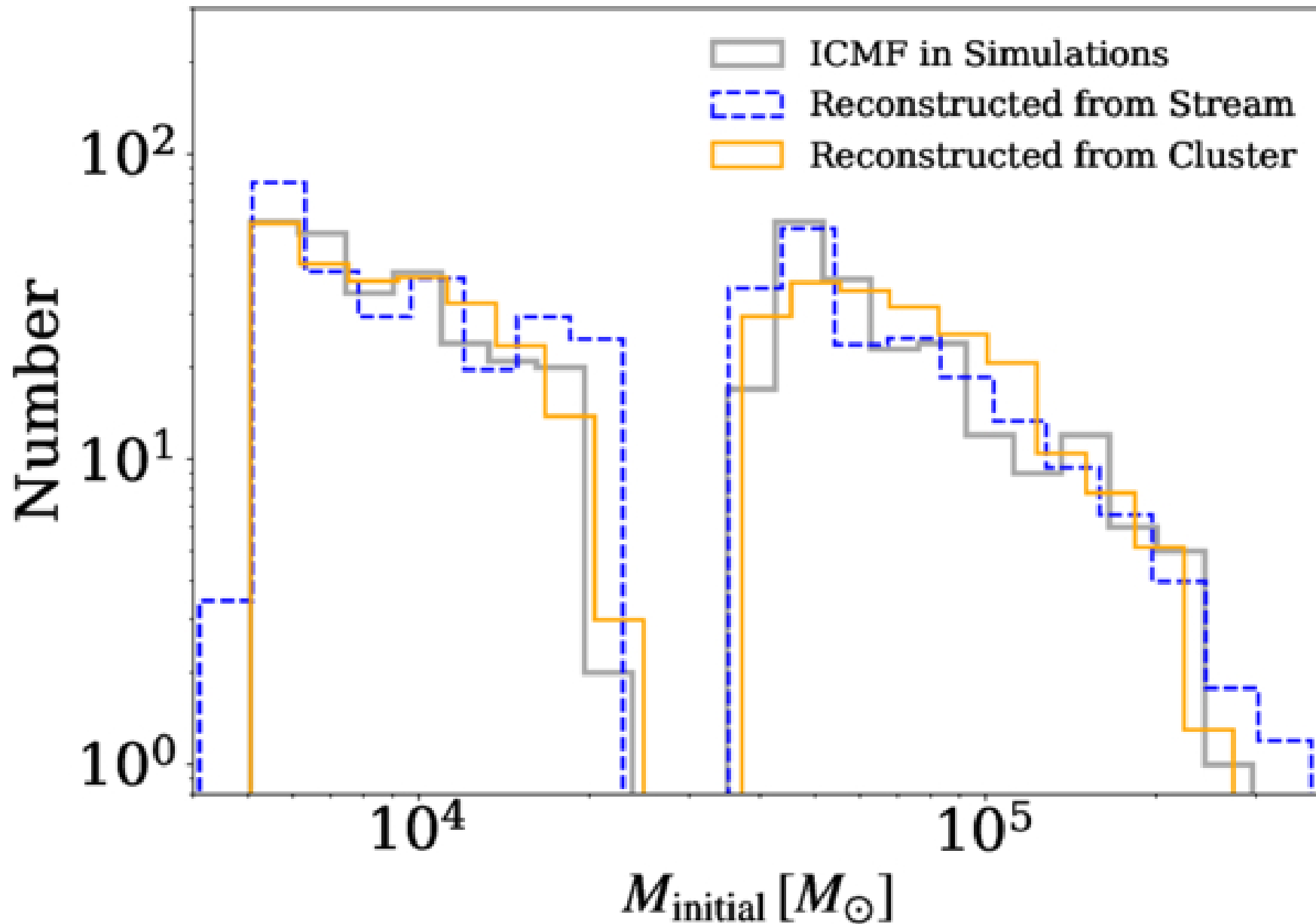
Figure 8. from Claire S. Ye and Raymond G. Carlberg 2026 Astrophys. J. Lett. 1007 doi:10.3847/2041-8213/ae8d0f https://dx.doi.org/10.3847/2041-8213/ae8d0f © 2026. The Author(s). Published by the American Astronomical Society.
