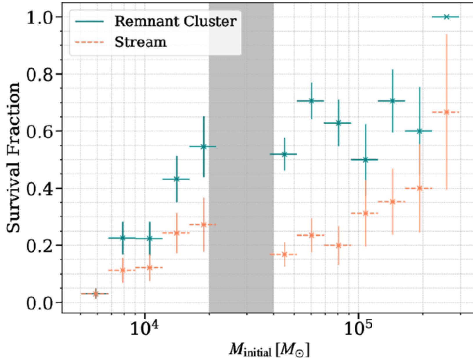
Figure 7. from Claire S. Ye and Raymond G. Carlberg 2026 Astrophys. J. Lett. 1007 doi:10.3847/2041-8213/ae8d0f https://dx.doi.org/10.3847/2041-8213/ae8d0f © 2026. The Author(s). Published by the American Astronomical Society.
