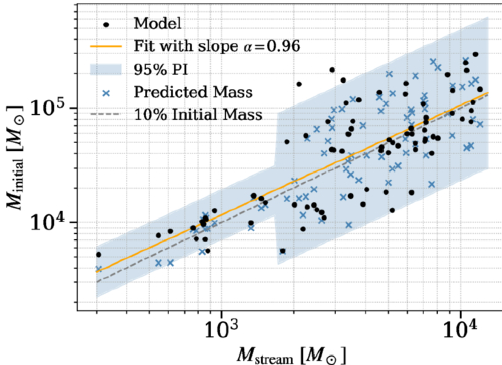
Figure 5. from Claire S. Ye and Raymond G. Carlberg 2026 Astrophys. J. Lett. 1007 doi:10.3847/2041-8213/ae8d0f https://dx.doi.org/10.3847/2041-8213/ae8d0f © 2026. The Author(s). Published by the American Astronomical Society.
