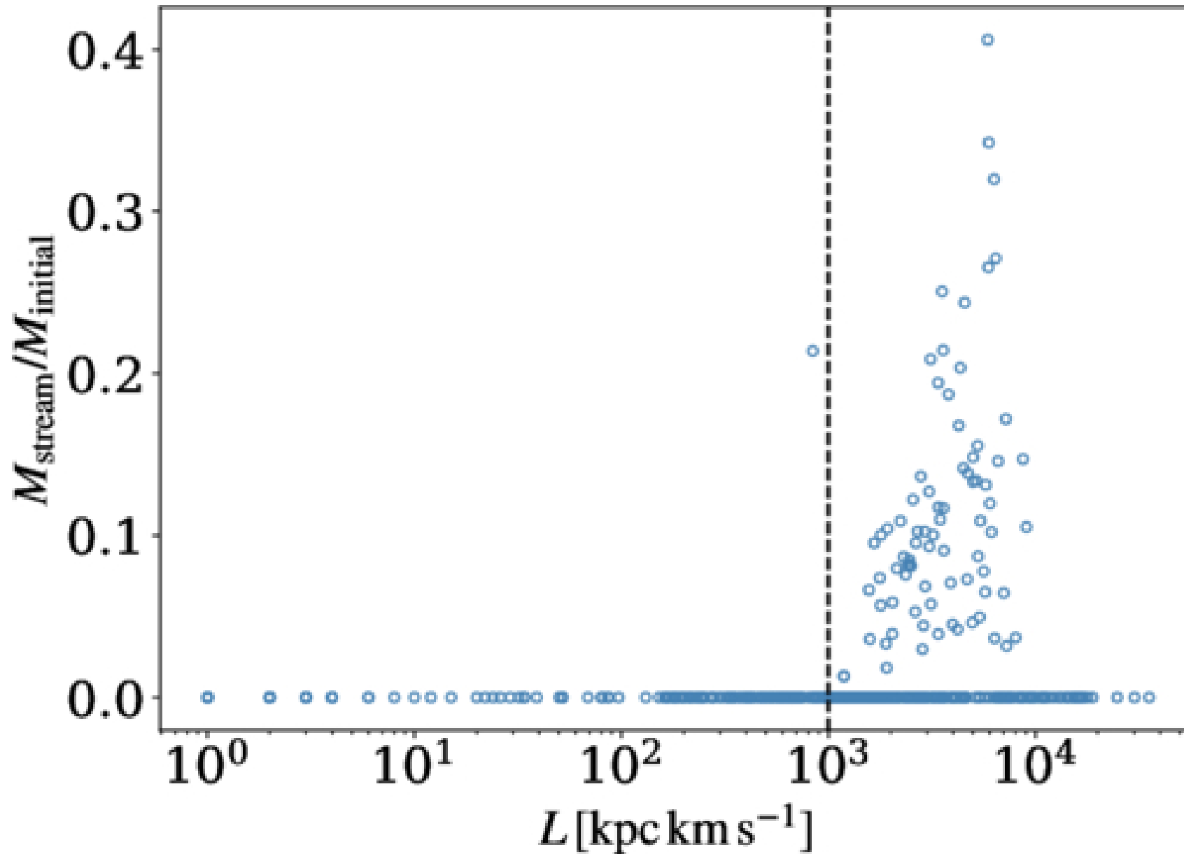
Figure 2. from Claire S. Ye and Raymond G. Carlberg 2026 Astrophys. J. Lett. 1007 doi:10.3847/2041-8213/ae8d0f https://dx.doi.org/10.3847/2041-8213/ae8d0f © 2026. The Author(s). Published by the American Astronomical Society.
