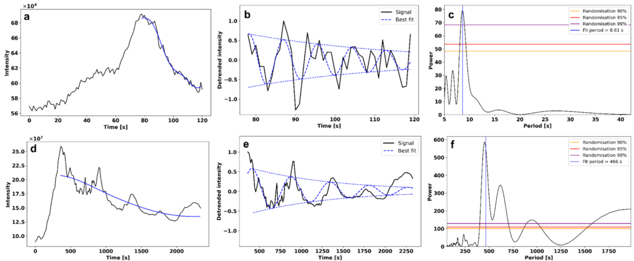
Figure 2. from Daye Lim et al 2026 Astrophys. J. Lett. 1007 doi:10.3847/2041-8213/ae8cfd https://dx.doi.org/10.3847/2041-8213/ae8cfd © 2026. The Author(s). Published by the American Astronomical Society.
