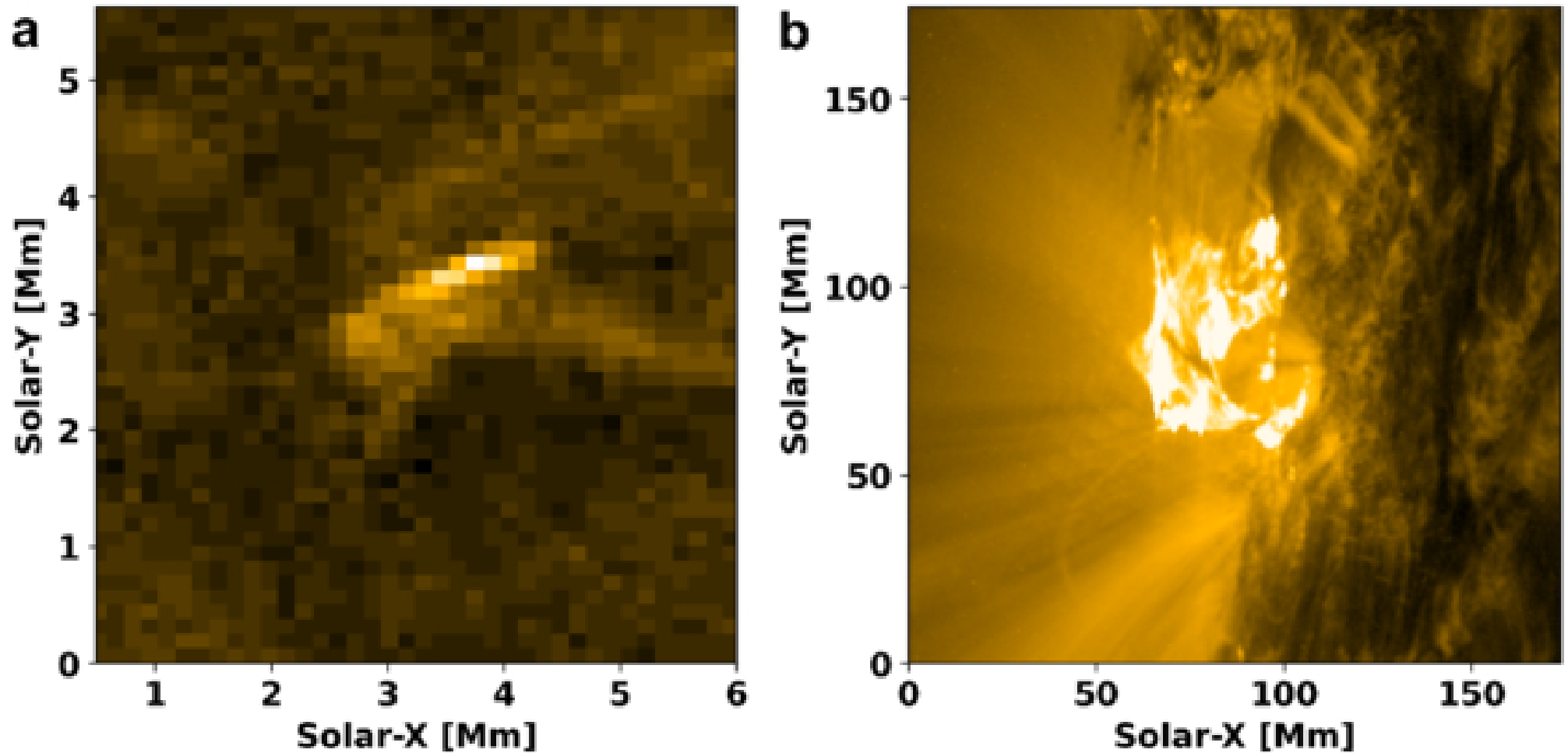
Figure 1. from Daye Lim et al 2026 Astrophys. J. Lett. 1007 doi:10.3847/2041-8213/ae8cfd https://dx.doi.org/10.3847/2041-8213/ae8cfd © 2026. The Author(s). Published by the American Astronomical Society.
