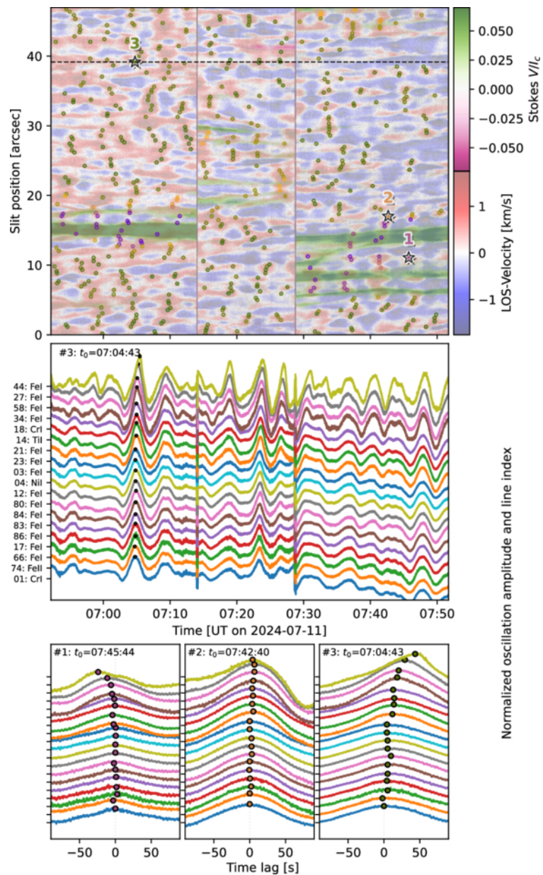
Figure 4. from Andreas Lagg et al 2026 Astrophys. J. Lett. 1007 doi:10.3847/2041-8213/ae8cfa https://dx.doi.org/10.3847/2041-8213/ae8cfa © 2026. The Author(s). Published by the American Astronomical Society.
