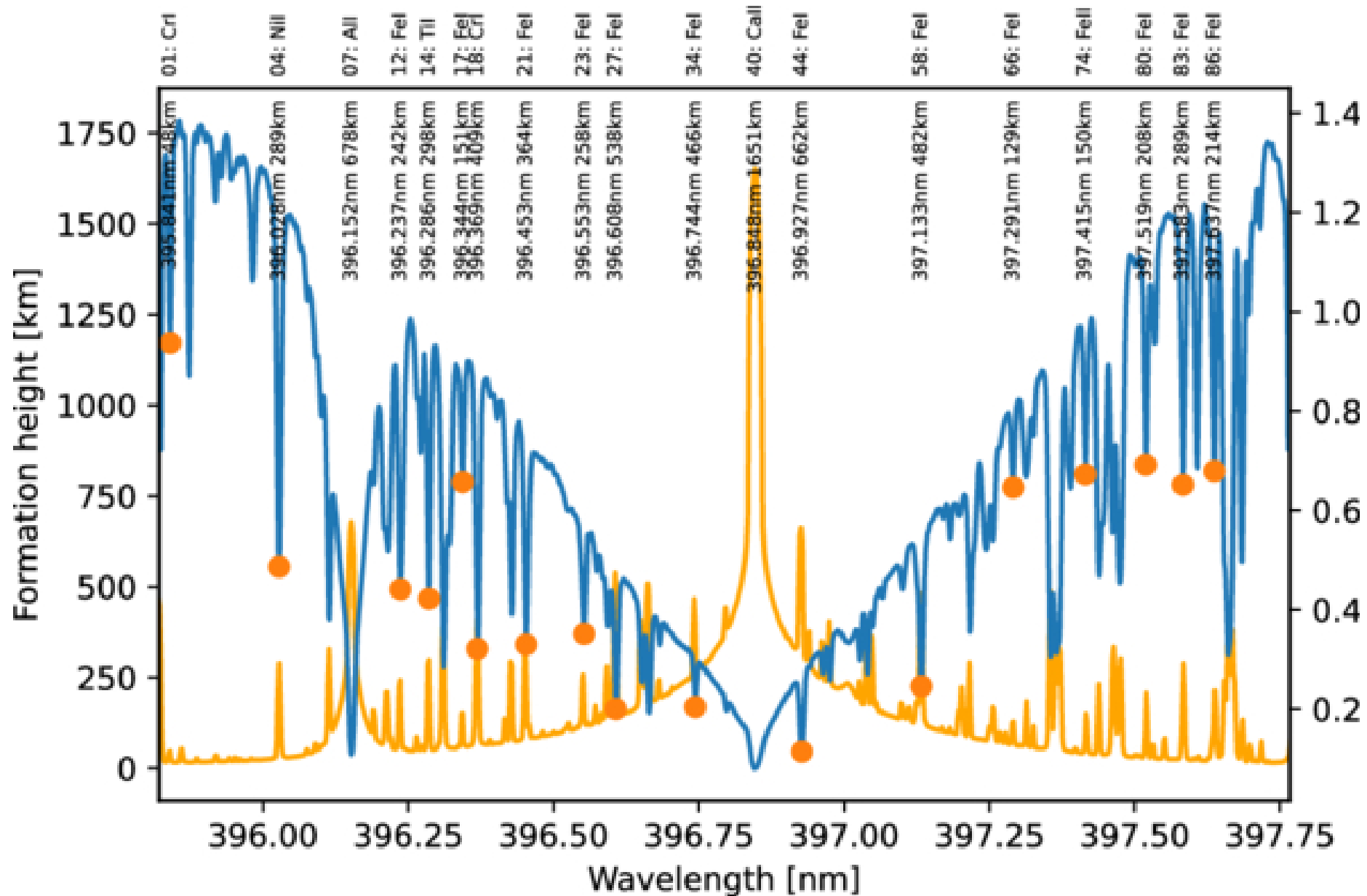
Figure 3. from Andreas Lagg et al 2026 Astrophys. J. Lett. 1007 doi:10.3847/2041-8213/ae8cfa https://dx.doi.org/10.3847/2041-8213/ae8cfa © 2026. The Author(s). Published by the American Astronomical Society.
