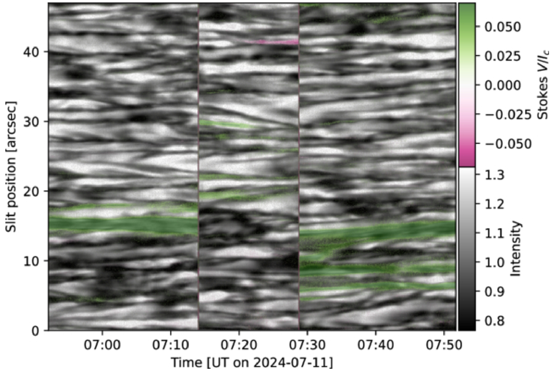
Figure 2. from Andreas Lagg et al 2026 Astrophys. J. Lett. 1007 doi:10.3847/2041-8213/ae8cfa https://dx.doi.org/10.3847/2041-8213/ae8cfa © 2026. The Author(s). Published by the American Astronomical Society.
