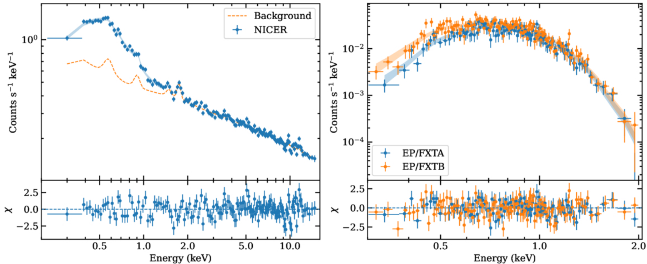
Figure 2. from Rahul Sharma et al 2026 Astrophys. J. Lett. 1007 doi:10.3847/2041-8213/ae8cf7 https://dx.doi.org/10.3847/2041-8213/ae8cf7 © 2026. The Author(s). Published by the American Astronomical Society.
