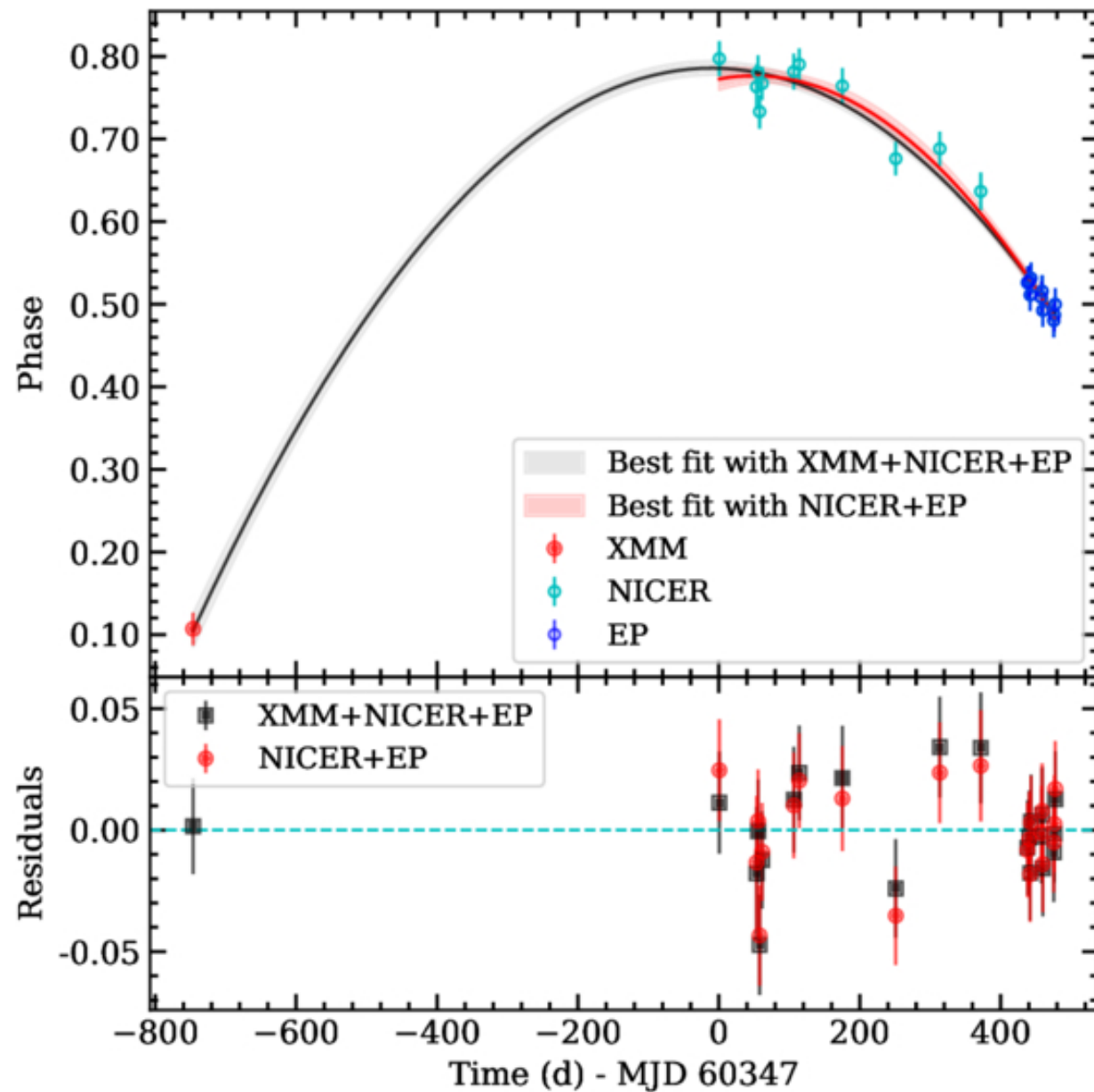
Figure 1. from Rahul Sharma et al 2026 Astrophys. J. Lett. 1007 doi:10.3847/2041-8213/ae8cf7 https://dx.doi.org/10.3847/2041-8213/ae8cf7 © 2026. The Author(s). Published by the American Astronomical Society.
