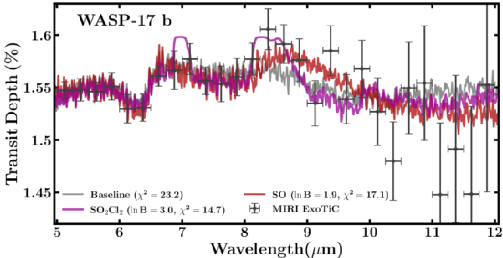
Figure 9. from Martin Binet et al 2026 Astrophys. J. Lett. 1008 doi:10.3847/2041-8213/ae8c2d https://dx.doi.org/10.3847/2041-8213/ae8c2d © 2026. The Author(s). Published by the American Astronomical Society.
