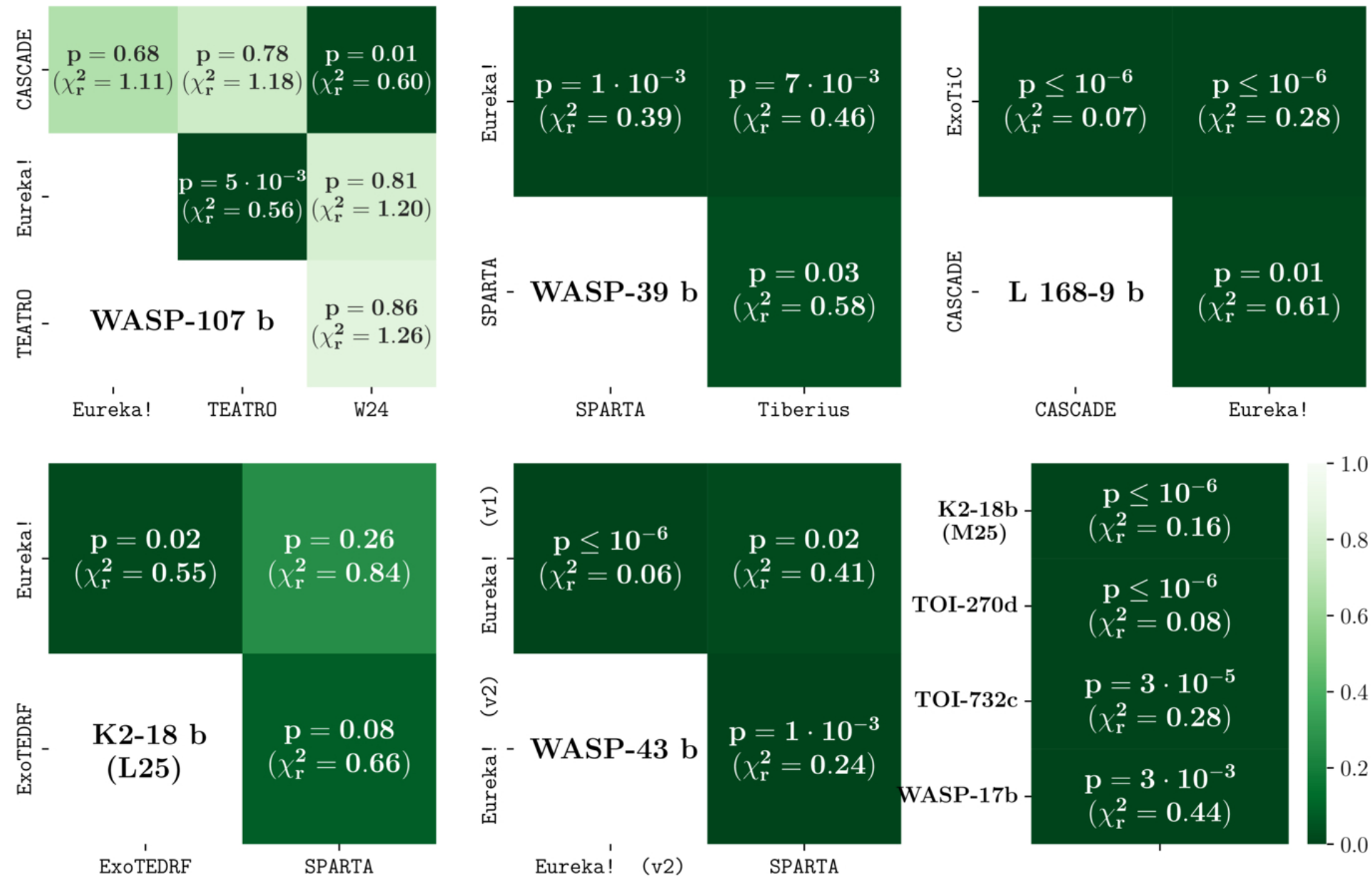
Figure 6. from Martin Binet et al 2026 Astrophys. J. Lett. 1008 doi:10.3847/2041-8213/ae8c2d https://dx.doi.org/10.3847/2041-8213/ae8c2d © 2026. The Author(s). Published by the American Astronomical Society.
