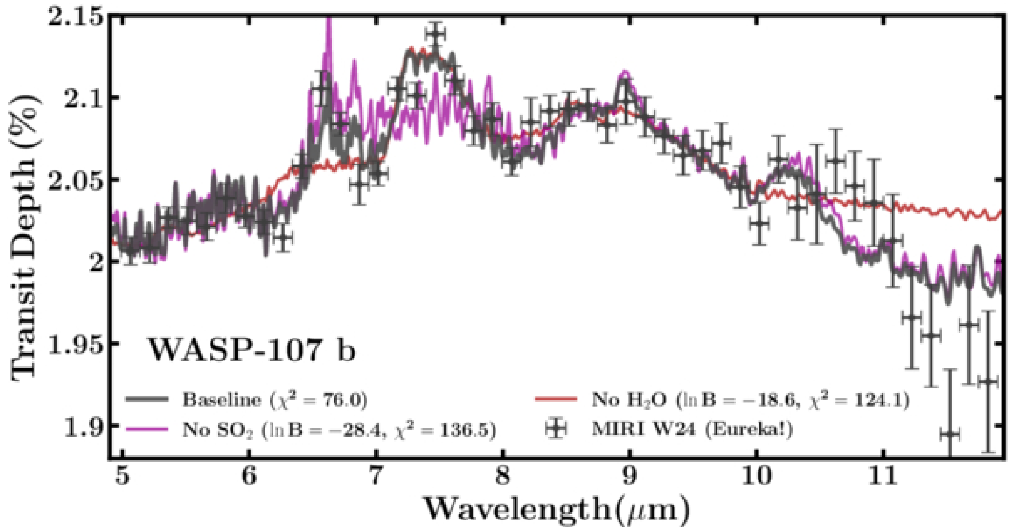
Figure 17. from Martin Binet et al 2026 Astrophys. J. Lett. 1008 doi:10.3847/2041-8213/ae8c2d https://dx.doi.org/10.3847/2041-8213/ae8c2d © 2026. The Author(s). Published by the American Astronomical Society.
