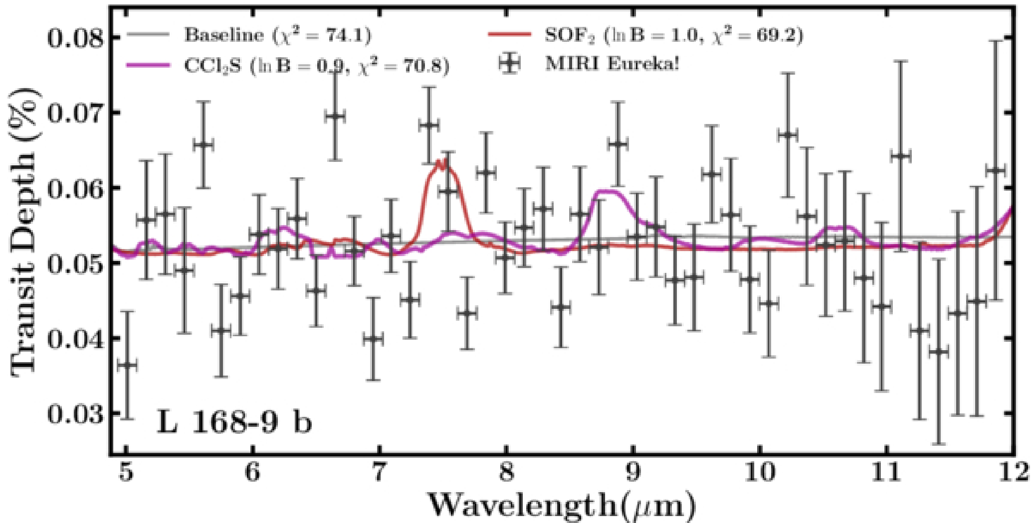
Figure 12. from Martin Binet et al 2026 Astrophys. J. Lett. 1008 doi:10.3847/2041-8213/ae8c2d https://dx.doi.org/10.3847/2041-8213/ae8c2d © 2026. The Author(s). Published by the American Astronomical Society.
